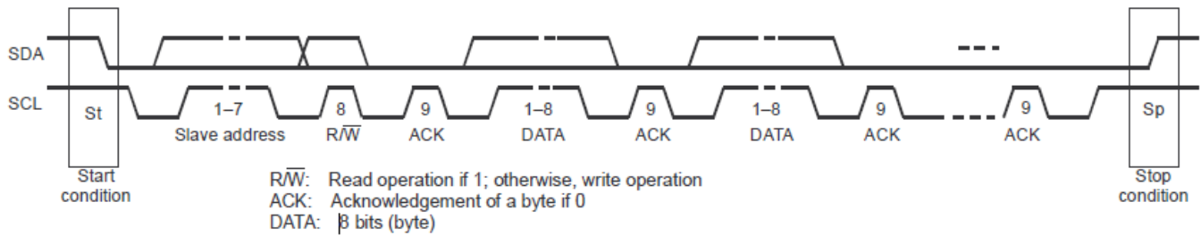
Figure 49. Packet Protocol
