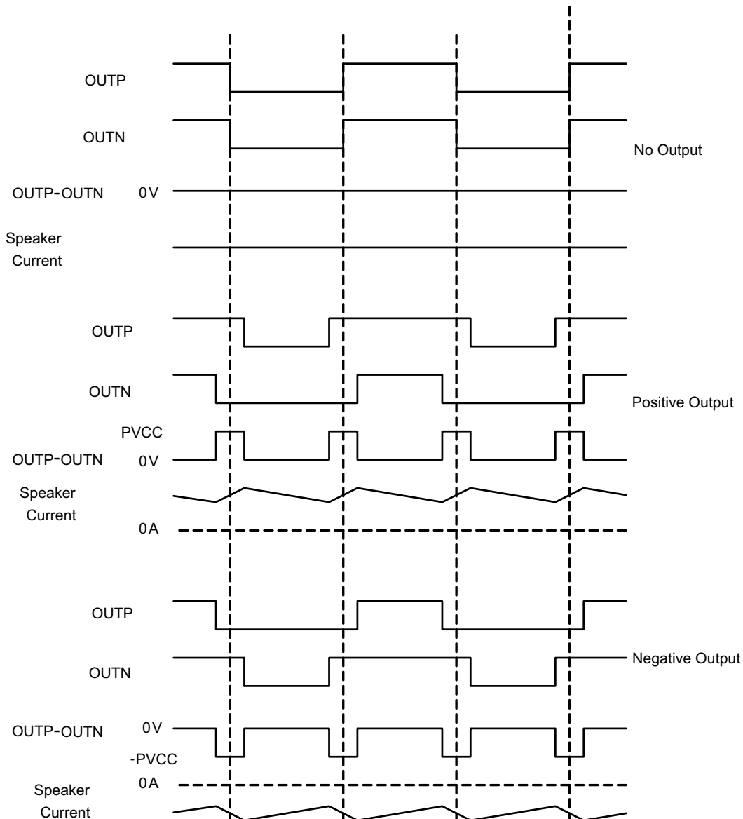
Figure 31. BD-Modulation
