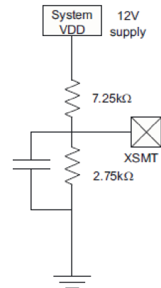
Figure 46. External Power Sense
