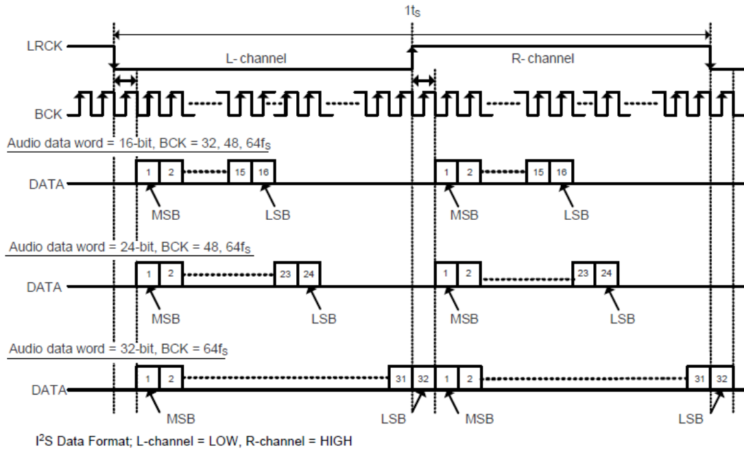
Figure 39. I 2 S Audio Data Format
