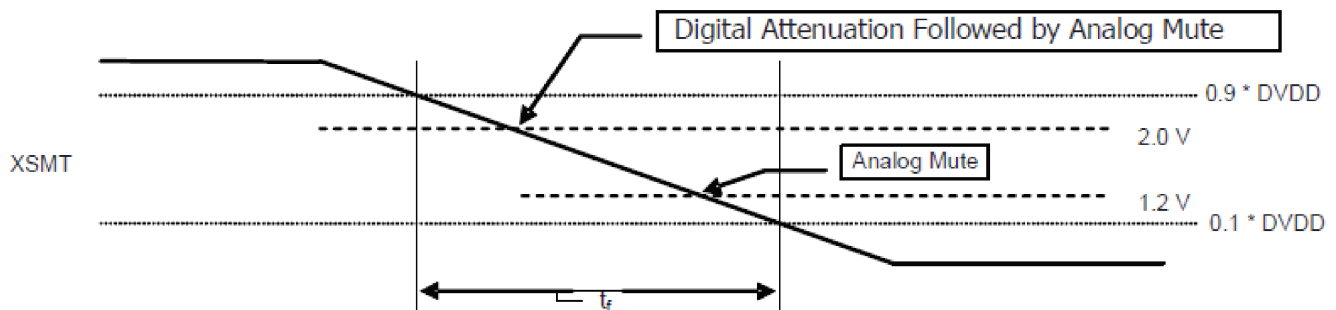
Figure 47. XSMT Timing for Undervoltage Protection
