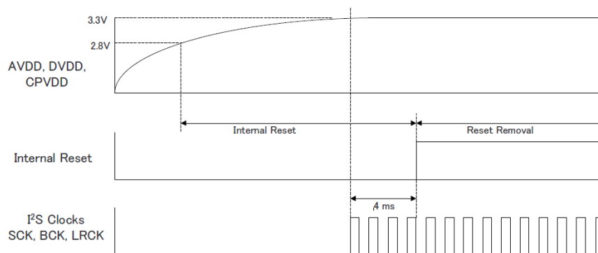
Figure 33. Power-On Reset Timing, DVDD = 3.3V
