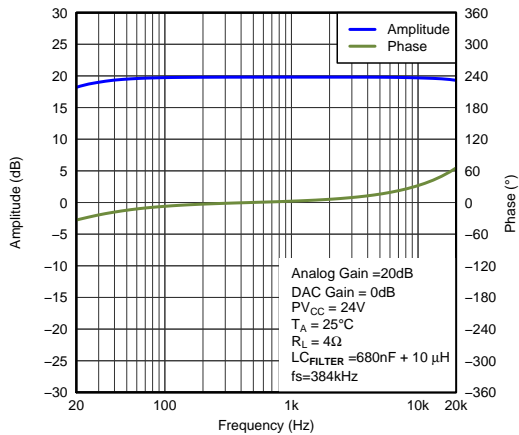
Figure 52. Gain/Phase vs Frequency
